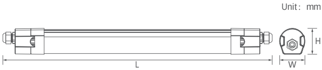
Unit: mm
