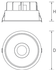
Unit: mm
